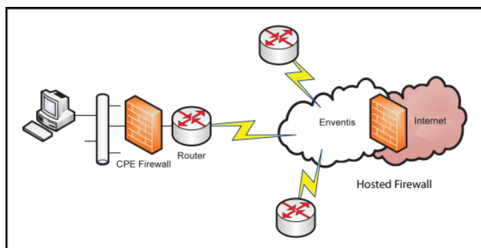
Hosted Firewall in conjunction with customer's existing firewall
